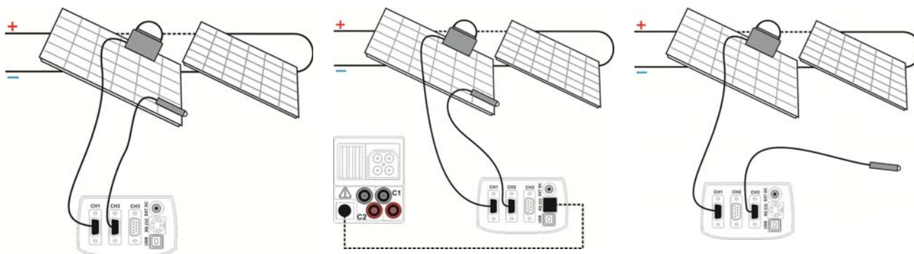
Figure 5-2: Measurement of environmental parameters
